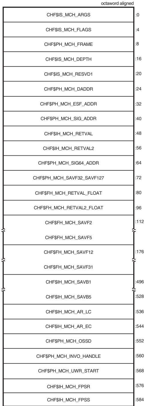
Figure 9–11 I64 Mechanism Vector Format
