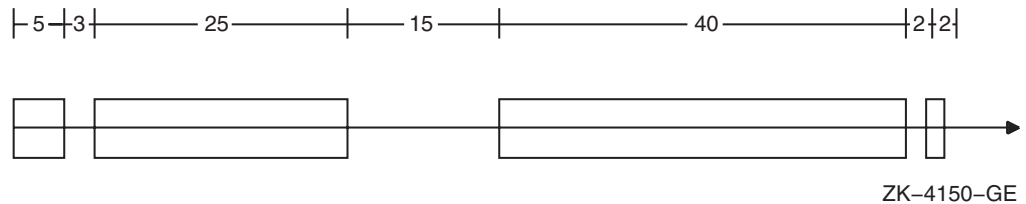
Figure 14–1 Memory Fragmentation
