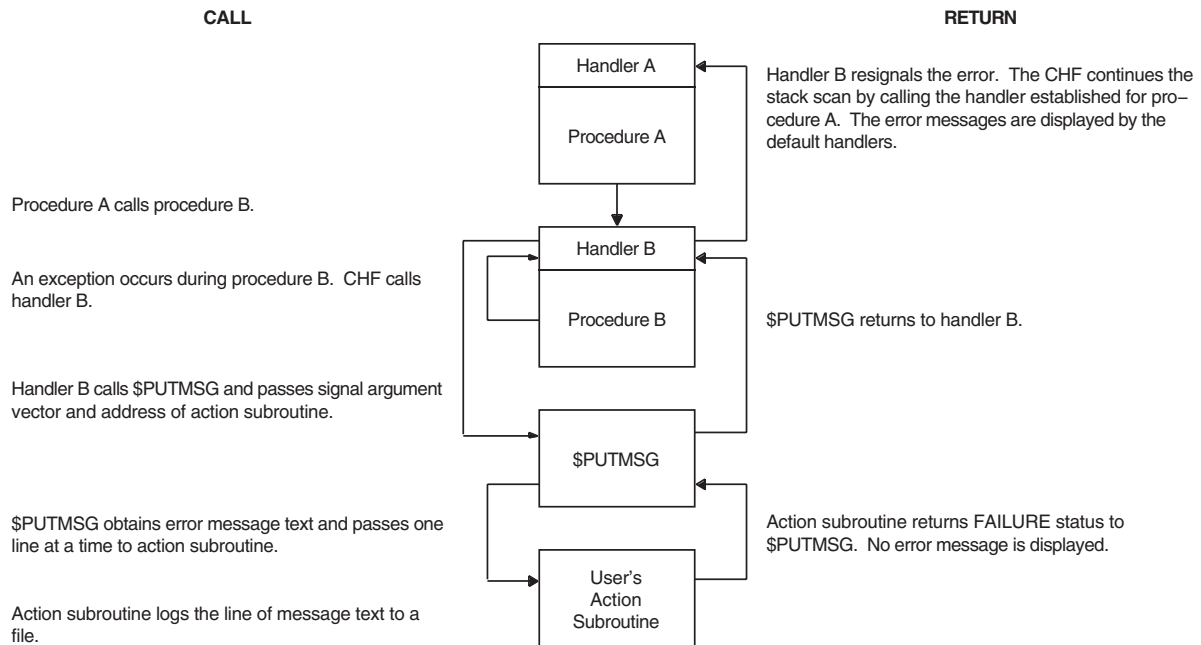
Figure 9–16 Using a Condition Handler to Log an Error Message
