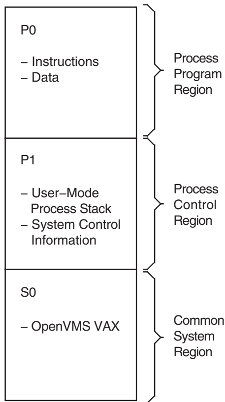
Figure 13–1 Virtual Address Overview on VAX Systems
