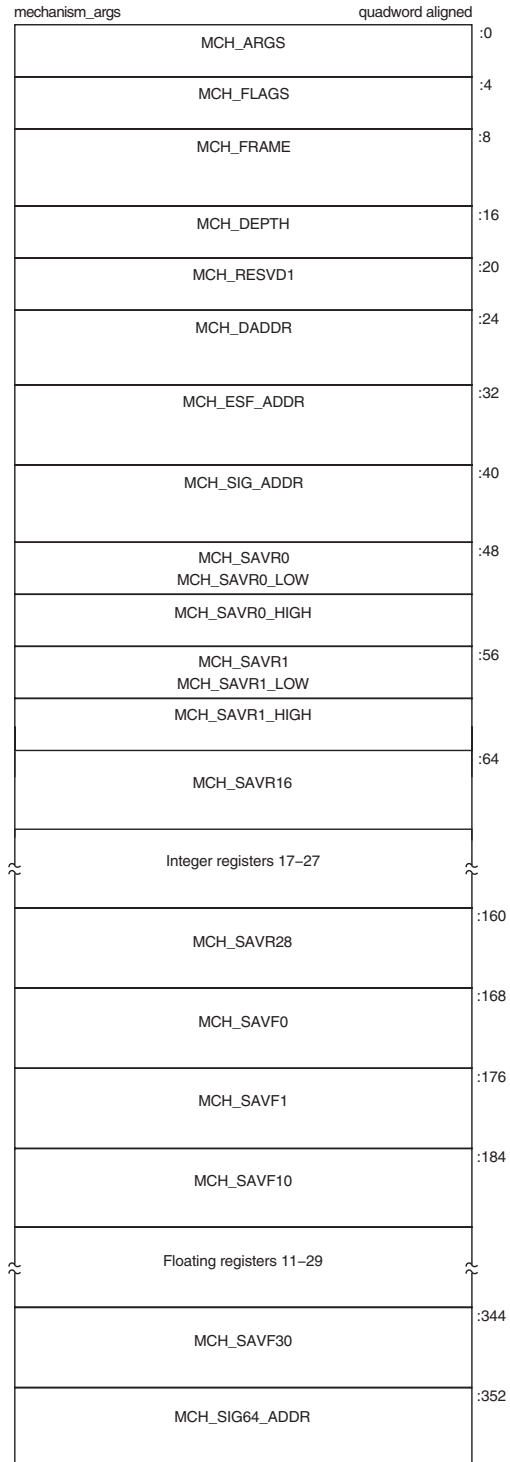
Figure 9–10 Mechanism Array on Alpha Systems
