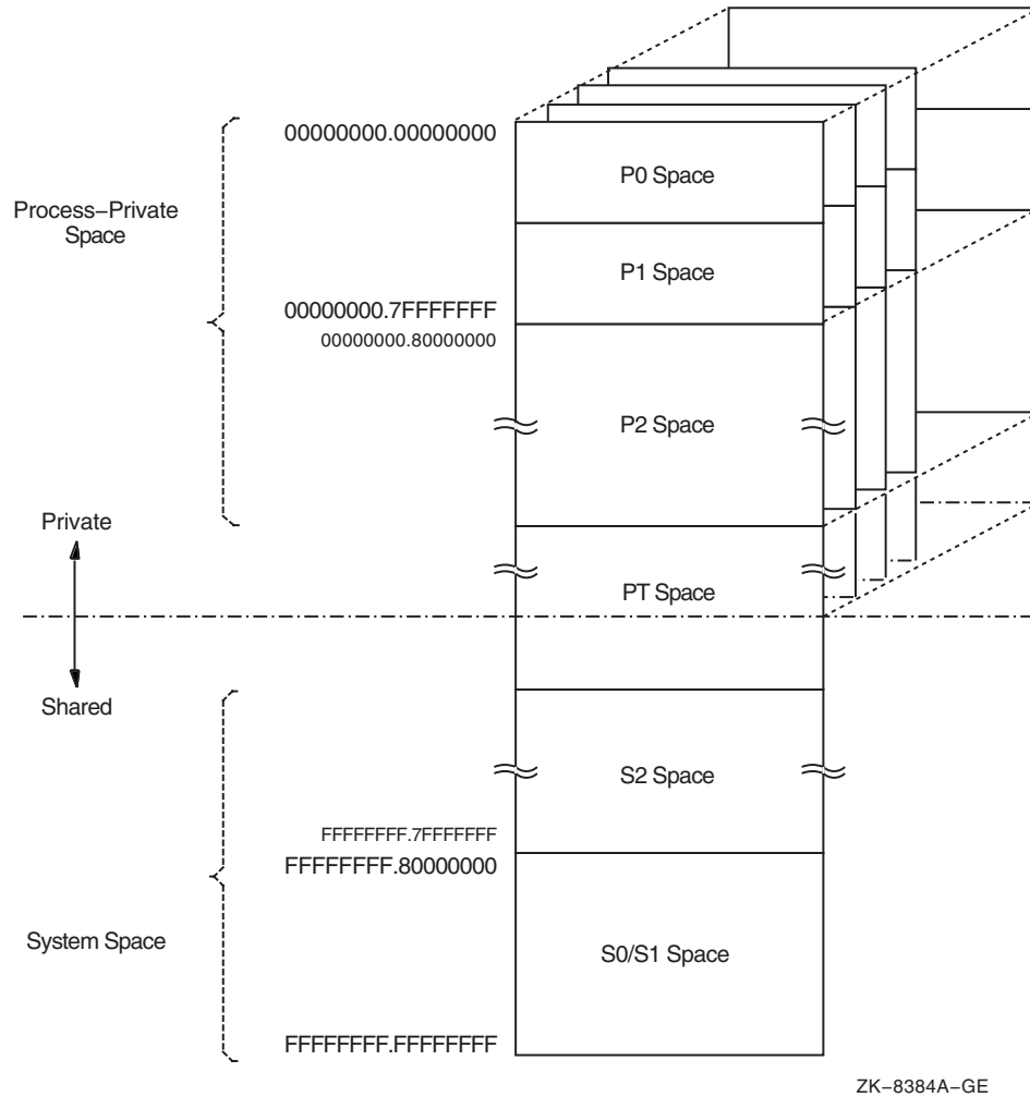
Figure 10–2 64-Bit Virtual Address Space Layout
