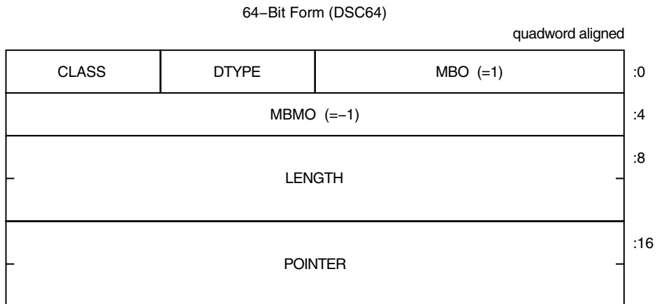
Figure 11–2 General Format of a 64-Bit Descriptor
