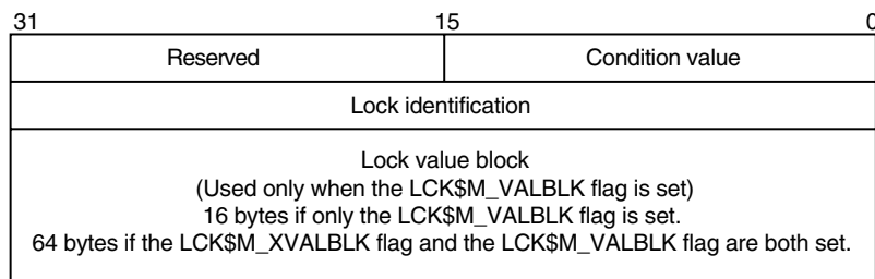
Figure 7–4 Lock Status Block
