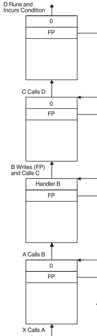
Figure 9–14 Unwinding the Call Stack
