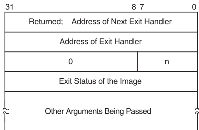
Figure 9–17 Structure of an Exit Handler
